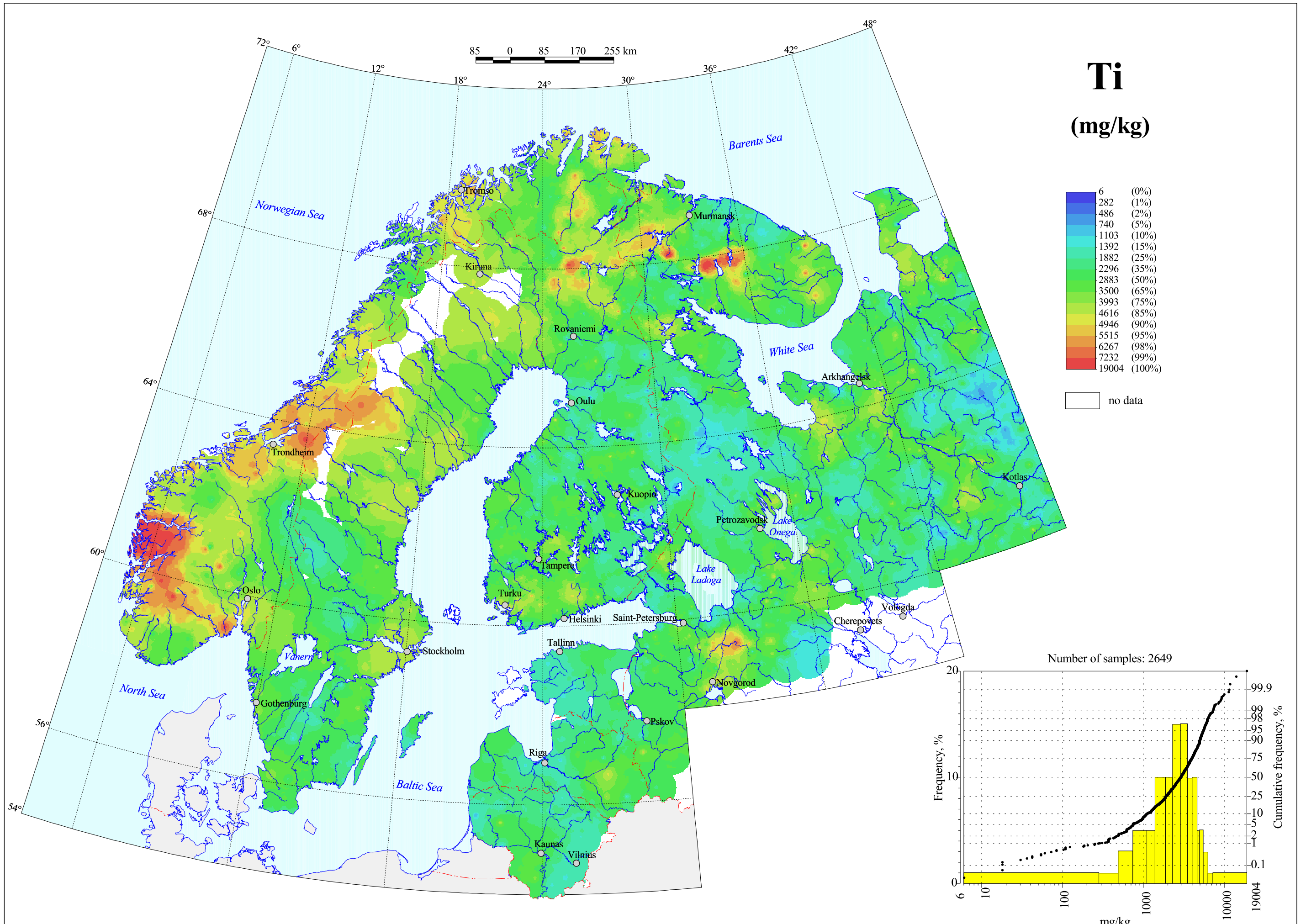
Titanium in C-horizon, Grain Size <2 mm, Total Content
